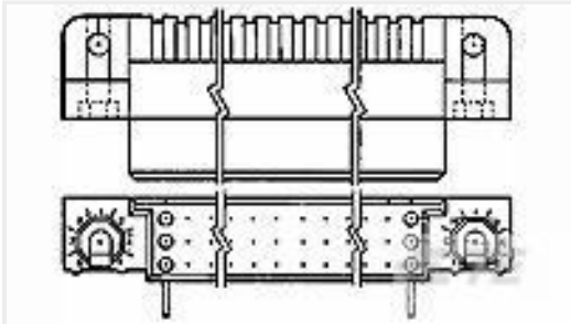
TE 产品编号212059-1 RECPT ASSY,SZ 3,AMPLIMITE COAX
