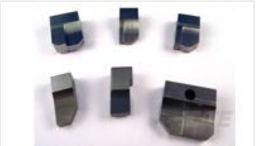
TE 产品编号2-1633128-3 ANVIL, COMBINATION .055
