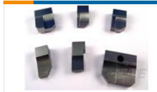
TE 产品编号2-662183-0 ANVIL, COMBINATION .055
