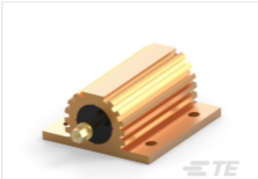
TE 产品编号2-2176731-0 HSC100S 2R2 5% Screw Terminal
