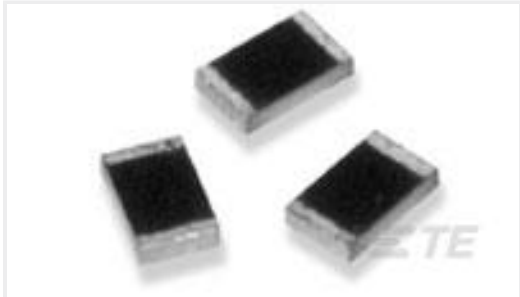
TE 产品编号6-1879744-3 RP 1J 226R 0.1% 15PPM CUT LENGTH
