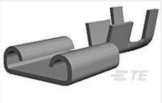
TE 产品编号 4-160256-2 250 FASTON,REC.,17-14 AWG,PNST
