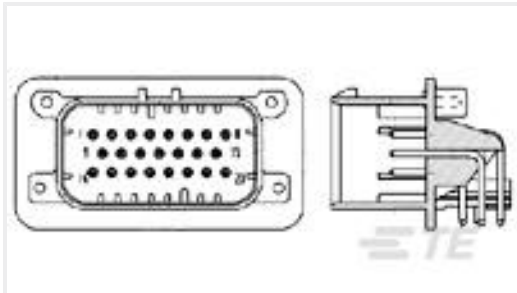
TE 产品编号1-776267-1 14POS,PIN DIA 1.3,HDR ASSY,90DEG, COD 1
