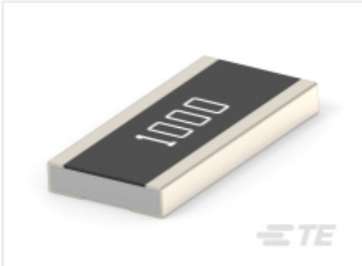
TE 产品编号1-2176562-9 3430 H2 1% 5R1 150ppm 1k RL
