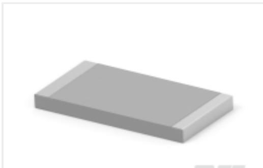
TE 产品编号5-2176331-6 CRGP 2512 390K 1%
