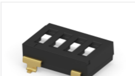
TE 产品编号2-2319747-1 TRI-STATE DIP 4P G RECESS T&R
