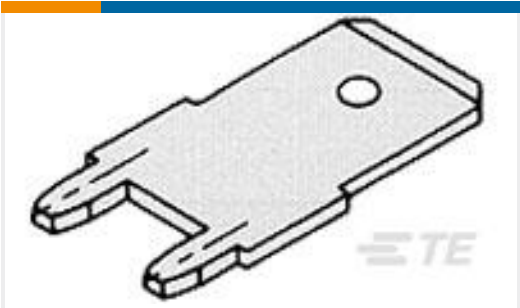
TE 产品编号62650-1 250 FASTON TAB TPBR
