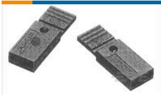
TE 产品编号881545-1 SHUNT LP W/HANDLE 2POS 15AU
