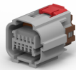
TE 产品编号1-1897168-3 0.64MM SLD 6(10)P PLUG ASSY-A GRY
