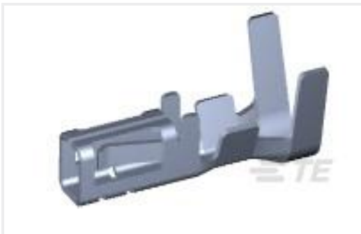
TE 产品编号1983780-1 NG GIC 3.3 REC CONTACT TIN PLATE
