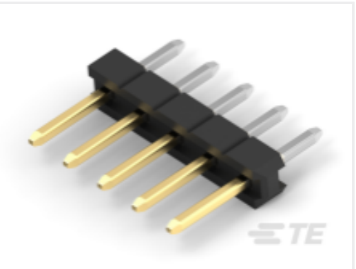
TE 产品编号2355172-5 5P,2MM,BRK HDR,SRVT,2.8,0.1AU,BOX
