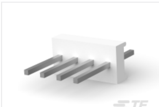
TE 产品编号CAT-104MTA-PVUNH PCB Header: Polyester, Vertical, Unshrouded, No Mating Alignment
