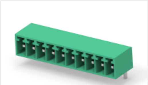
TE 产品编号1-2350514-0 10POS TB HDR 90 DEG, PITCH 3.5 &TL 3.5mm
