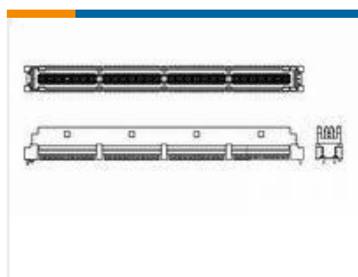
TE 产品编号2069917-2 V-P ASSY 12MM 160P IEX 0.8MM H-SP CONN.
