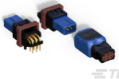
TE 产品编号YD369-B99-NS400000 369 9 WAY PANEL MNT REC, 90 PCB GOLD,SKT
