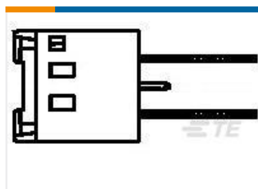
TE 产品编号1871845-3 GIC 2.5 ON TAPE HDR TIN VERSION 3P
