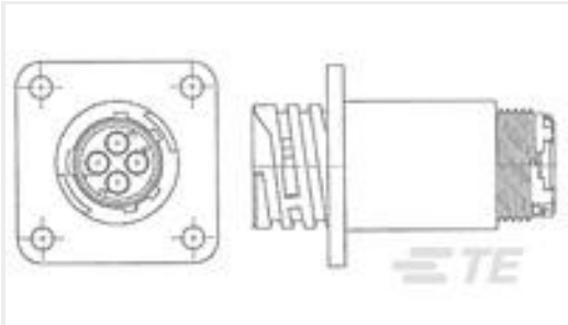
TE 产品编号788158-2 SLD CPC RCPT ASSY,13-9,STD SEX
