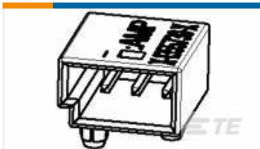
TE 产品编号1-1355730-1 3pos MQS .63 header 90deg
