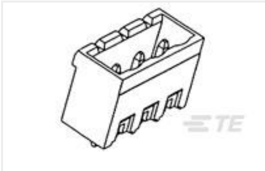
TE 产品编号796642-7 7POS 5.0MM CE VRT HDR,TRM BLK
