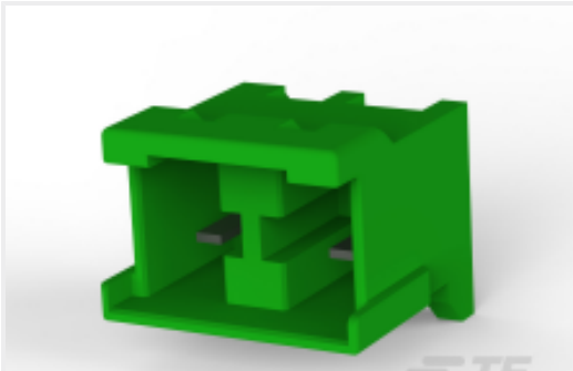
TE 产品编号1747052-5 GRACE INERTIA CONNECTOR 7.92 2POS HEADER
