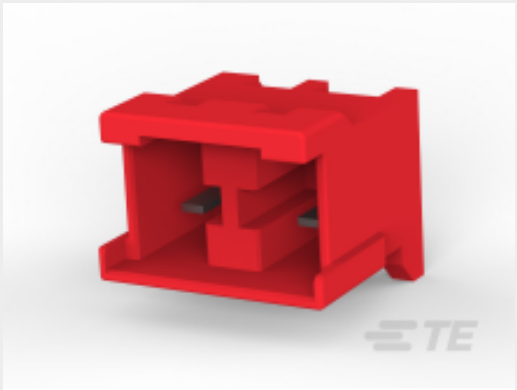
TE 产品编号1747052-2 GIC7.92 2POS_HEADER ASS'Y RED KEYING A
