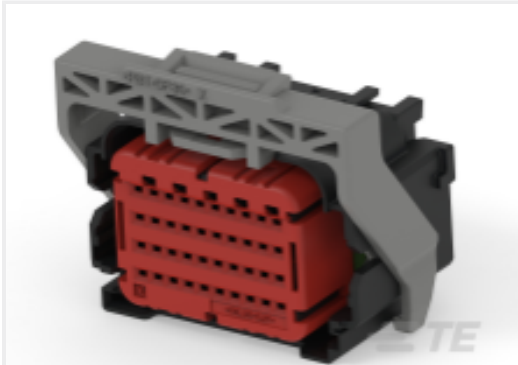
TE 产品编号5-1924513-4 GET 40 WAY HARNESS ASSY, KEY J
