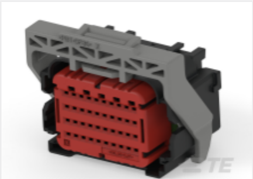
TE 产品编号5-1924513-3 GET 40 WAY HARNESS ASSY, KEY J
