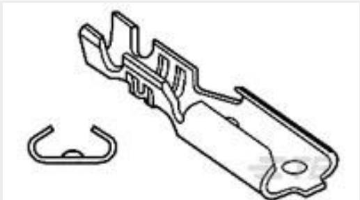
TE 产品编号60704-1 AMP EDGE TERM IS 20-18 016TPBR
