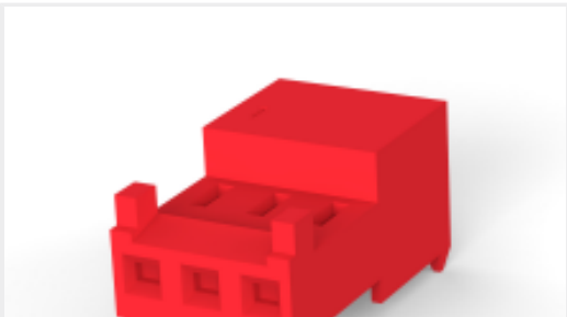
TE 产品编号CAT-104MTA-NTPMR Nylon Tin Plated Receptacle: 2.54 mm, with Mating Alignment, MTA 100
