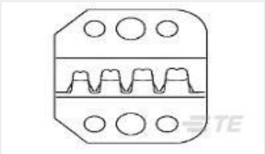
TE 产品编号58614-2 PROCRIMP, DIE, SL156
