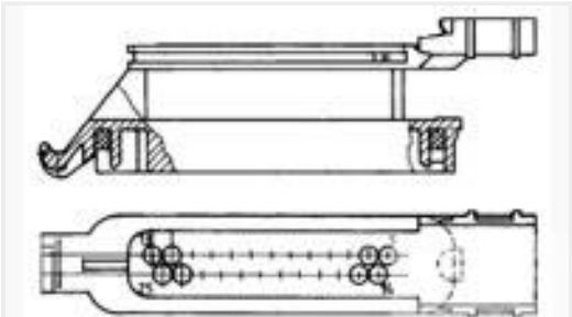
TE 产品编号CAT-D9934-A75 Contact: Component To Wire; 15A, 28-14 wire size
