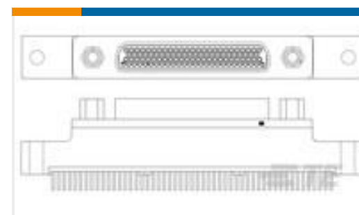
TE 产品编号 1532273-4 M83513/24-H01NP = MCKS-N1-S-100PST1
