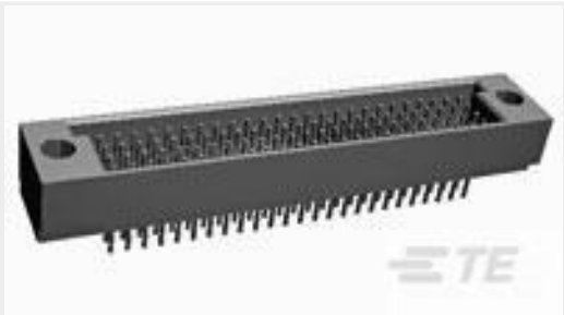
TE 产品编号532436-3 HDI PIN ASSY 4 ROW 128 POS
