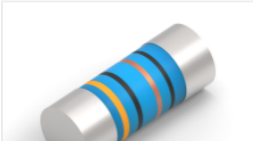
TE 产品编号8-2176316-9 MELF SMA-A 120K 1% 50PPM 0207 1W
