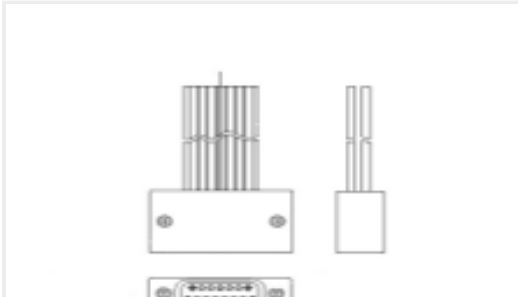
TE 产品编号8-1589476-0 STM015SC2DC036N = WDUALOBE
