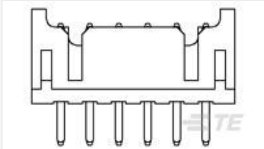
TE 产品编号1-1470109-6 2.0mm Pitch Header,Dip 16p
