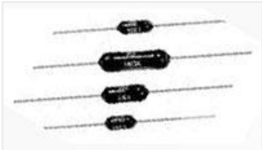
TE 产品编号5-1879663-5 H8 392R 0.1% 15PPM
