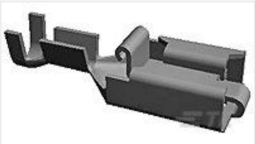
TE 产品编号170265-2 PL 250 REC 12-10 AWG 0.406 X 42.3
