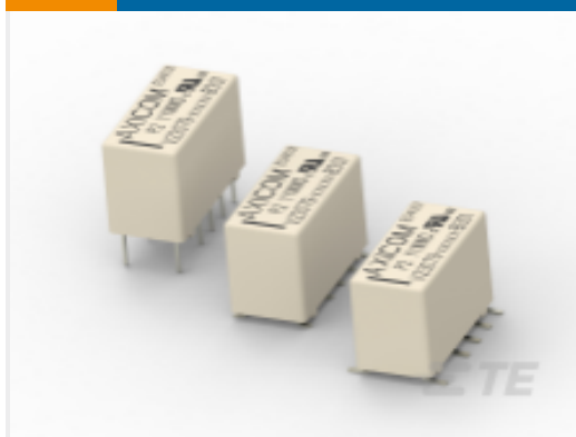
TE 产品编号 CAT-AX41-P1A Small Signal Relay, Axicom P2 Standard
