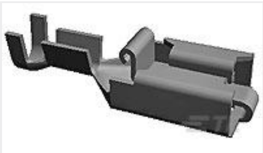
TE 产品编号927853-6 PL 250 REC TERMINAL 20-17 PTPB LP
