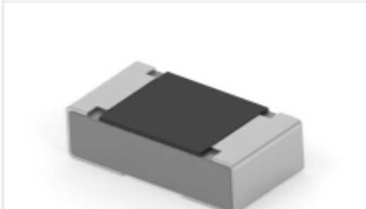
TE 产品编号7-2176479-1 RA73F 1J 274R 0.1% 5K RL
