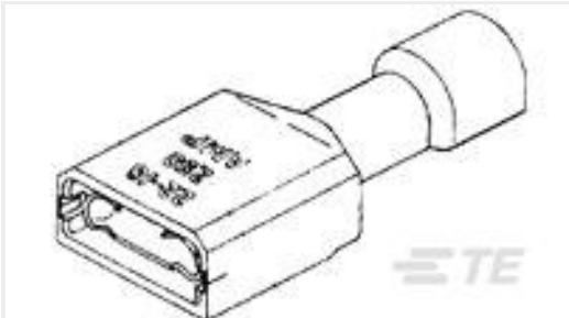
TE 产品编号4-520448-2 ULTRAFast 250 ASSY REC 12-10 TPBR LP
