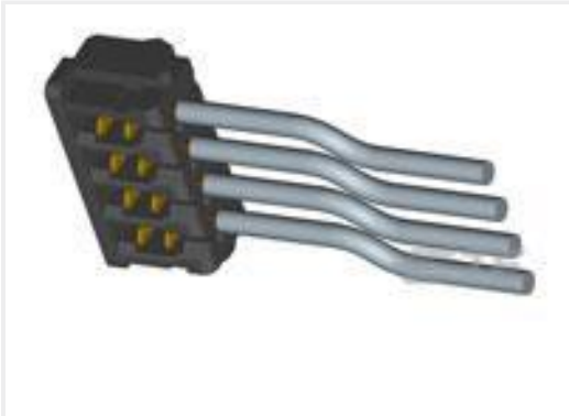
TE 产品编号 2-179694-4 CT MT REC ASSY 4P GRAY
