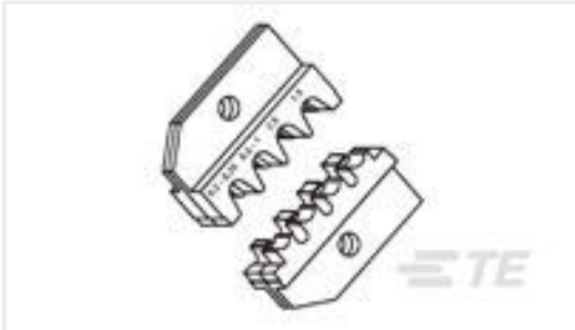
TE 产品编号160451-3 FF 250 TAB 18-14AWG PB SILVER PL LP
