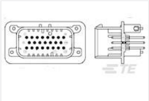
TE 产品编号776228-1 23POS,PIN DIA 1.3,HDR ASSY, 180DEG,COD 1
