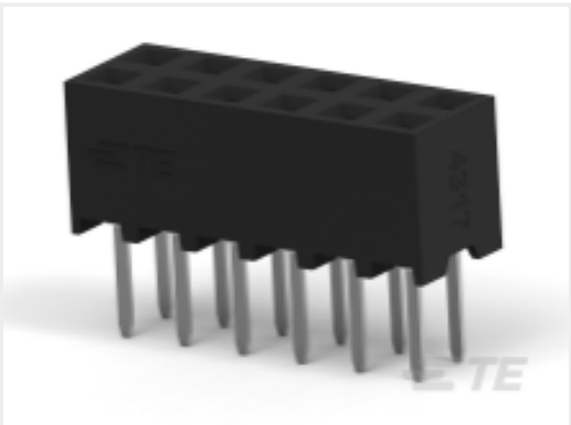
TE 产品编号 1-2314825-4 14P,2MM,B-B,REC,DRV,T,2.7,0.38AU,TB,W/CAP
