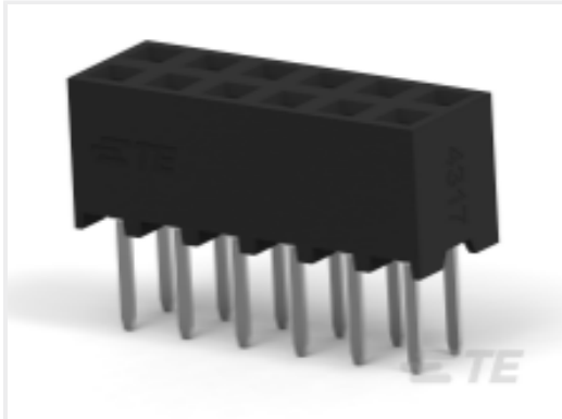
TE 产品编号 1-2314821-4 14P,2MM,B-B,REC,DRV,T,2.7,0.38AU,TB
