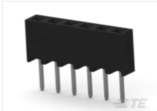
TE 产品编号 2307770-6 6P,2MM,BB,REC,SRVT,2.0,0.38AU,TR,W/CP
