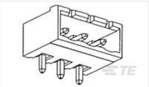
TE 产品编号796638-5 5POS 5.08MM CE R/A HDR,TRM BLK
