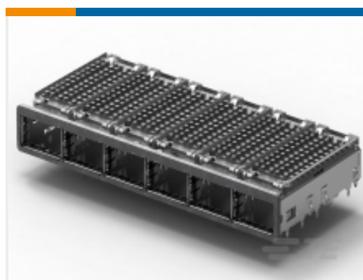
TE 产品编号 2143330-1 1X6 QSFP Kit Assy Bhd Bzl, PCI
