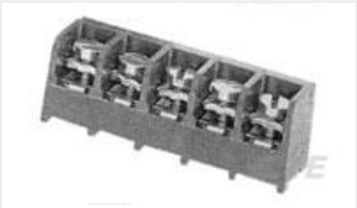
TE 产品编号1546833-3 .375", 3P, MOD W/ COVER
