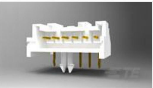
TE 产品编号1744426-2 Header Housing Assy, EP 2.5 RA, 2 Pos.
