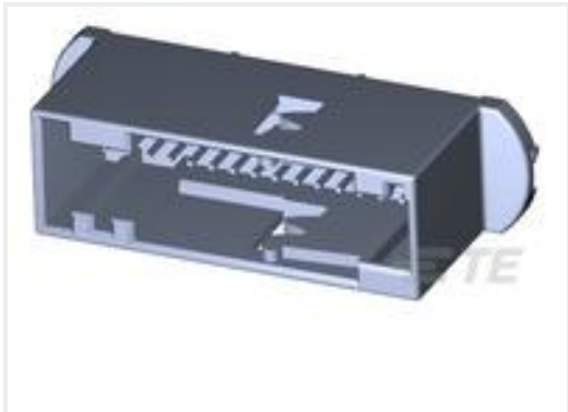
TE 产品编号2-966658-2 32pos MQS .63 header 180deg
