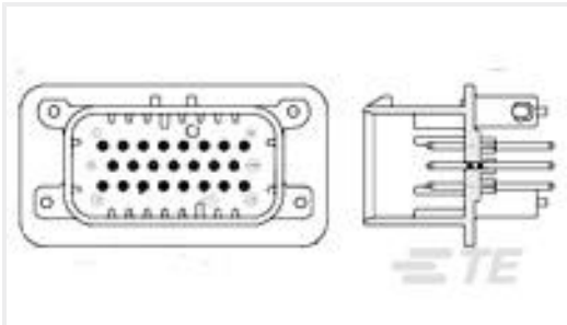
TE 产品编号1-776200-1 23POS,PIN DIA 1.3,HDR ASSY, 180DEG,COD 1
