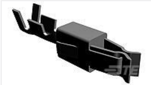
TE 产品编号965999-2 JPT A REC 2.8 Contact SRC Sn
