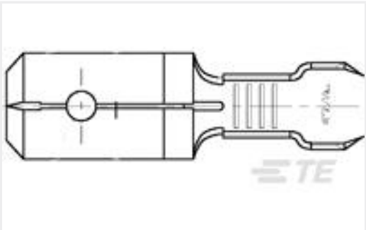
TE 产品编号60006-1 250 FASTON TAB 18-14 AWG BR
