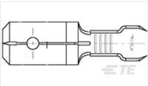
TE 产品编号60006-1 250 FASTON TAB 18-14 AWG BR
